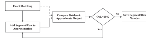
Fig. 2. Flow of ReCAM to determine approximate segments/rows.
