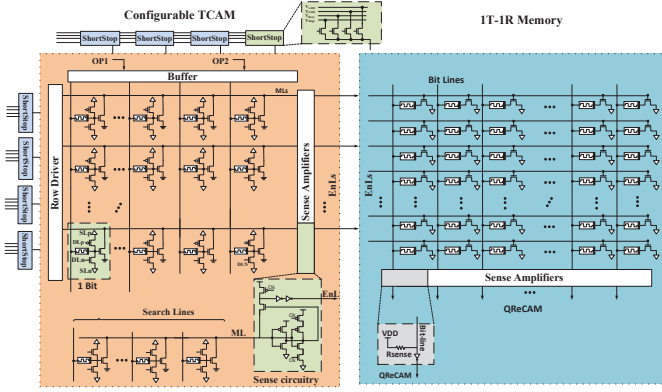
Fig. 1. ReCAM module architecture: 3T-1R TCAM plus 1T-1R memory.
